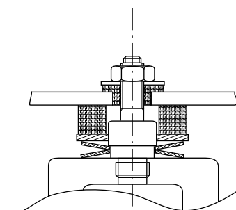
Unlock position transformer in use
